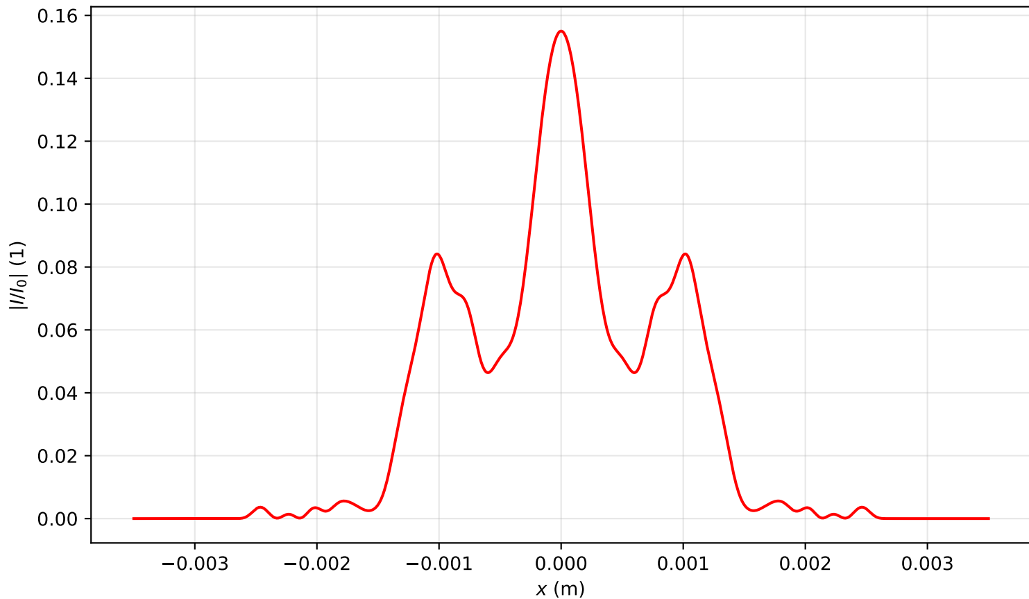
Intensity profile I(x, y = 0, z = 2.627)/I_0 , P_{in}=6.0P_{cr} , artificial time
